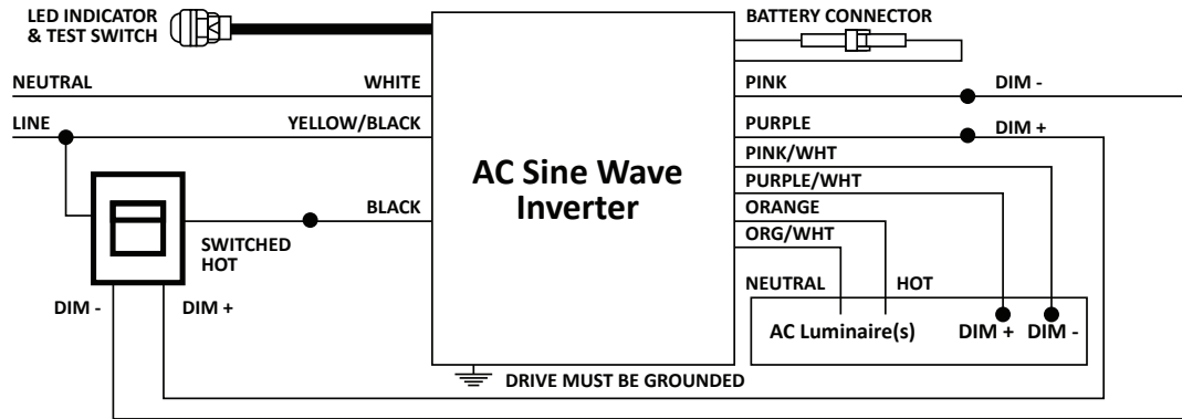
Figure A. Wiring Diagram with 0-10V Dimmer 175W Max. Connected Load
