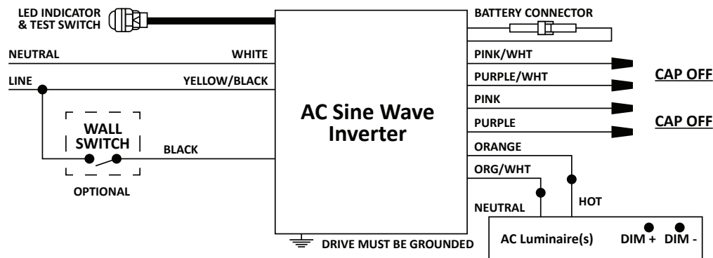
Figure B. Wiring Diagram without 0-10V Dimmer
